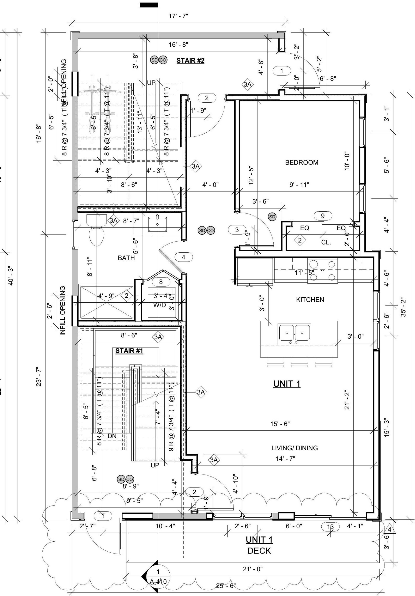
2 1ST FLOOR 1/4" = 1'-0"
