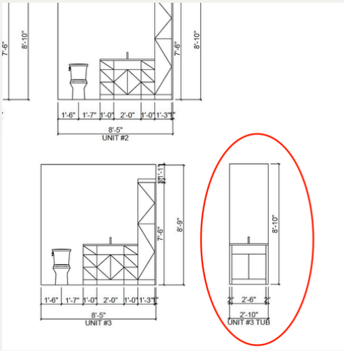
Vanity Elevation
