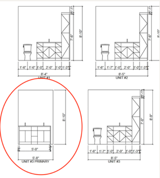
Vanity Elevation
