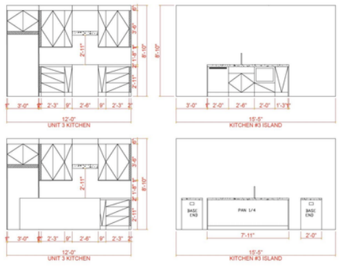
Kitchen Elevation
